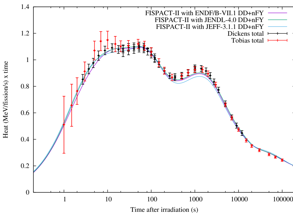
Figure 7: Simulation of thermal fission pulse on ^{239}\text{Pu} using variety of decay and nFY data, against experimental and statistical meta-analysis results.
