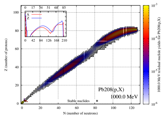
(13.4) 1 GeV
