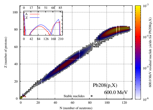
(13.2) 600 MeV
