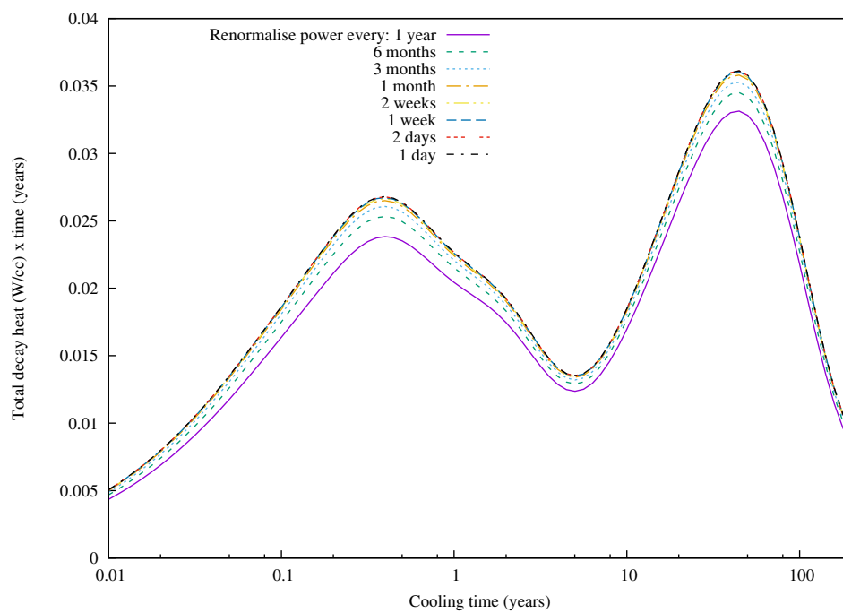
Figure 8: Comparison of the decay heat following a 1 year irradiation of LWR fuel with various periods for reaction rate re-calculation. The y-axis is given in \text{W}/\text{cm}^3 times the cooling time in years.
