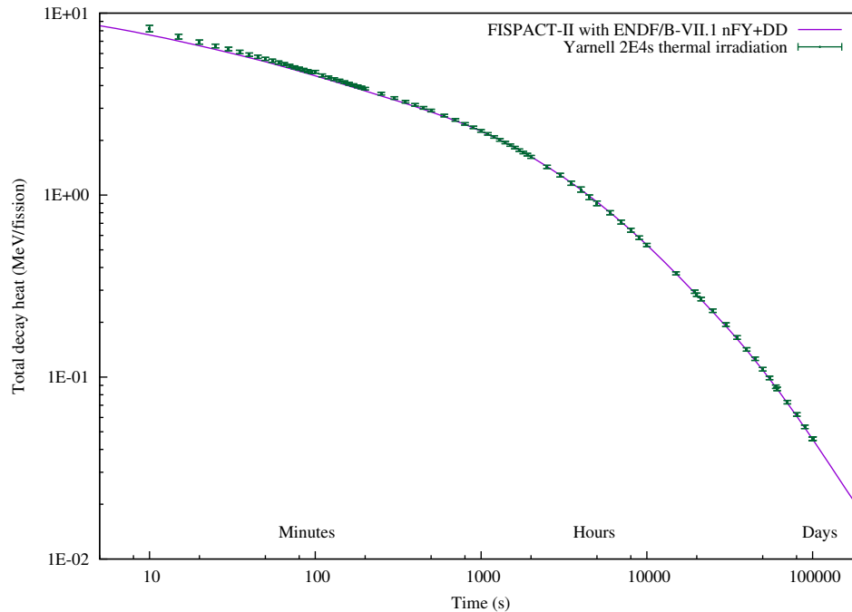
Figure 6: Simulation of 2.0 \times 10^4 s thermal fission of ^{235}\text{U} using ENDF/B-VII.1 decay and nFY data, against experimental calorimetric results.
