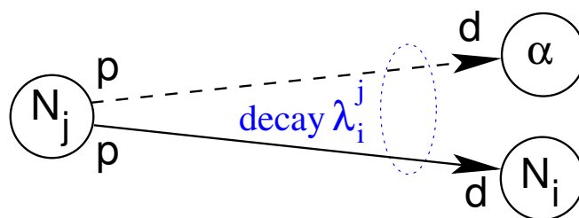
Figure 18: Decay processes (e.g., \alpha -decay) may produce secondary gas nuclides that are included in the inventory calculation.
