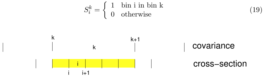
Figure 17: Projection operator S_i^k maps cross-section energy bins to covariance energy bins. The shaded energy bins have S_i^k = 1 , and all others have S_i^k = 0
